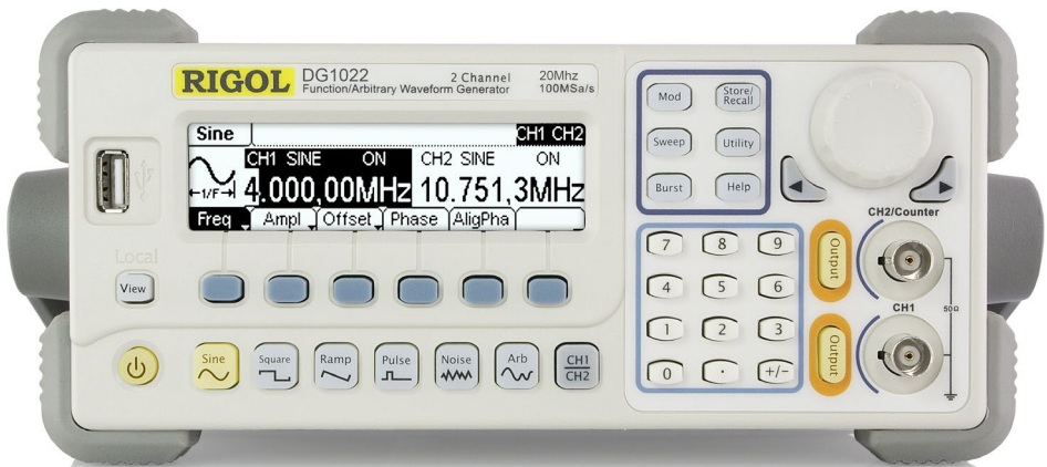
RIGOL DG1000(A)
